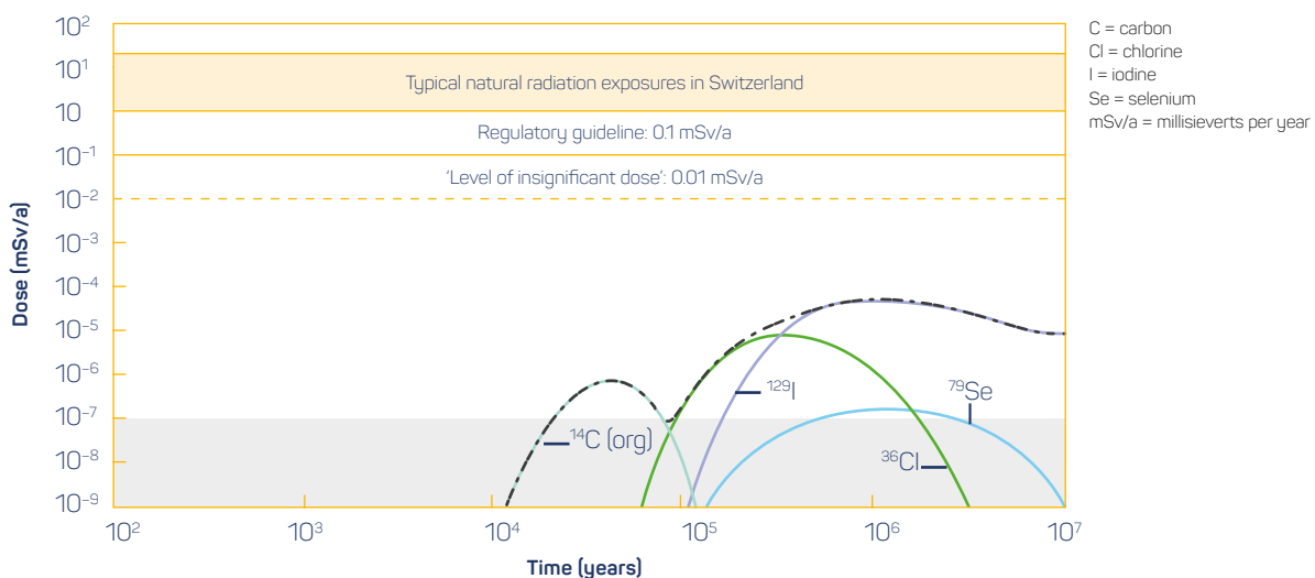
Figure I.3: Typical output of a safety assessment
