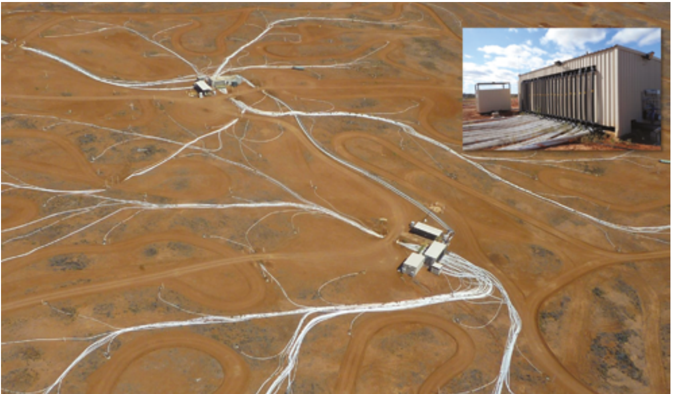
Figure 2.3: The Four Mile ISL wellfield, with inset showing pipework linking into a well-house
