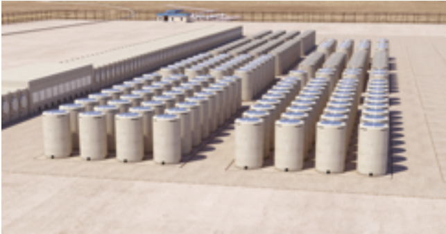
Figure 5.11: Dry cask storage facility, depicting casks stored in horizontally configured modules (left) and in a vertical configuration (centre)
