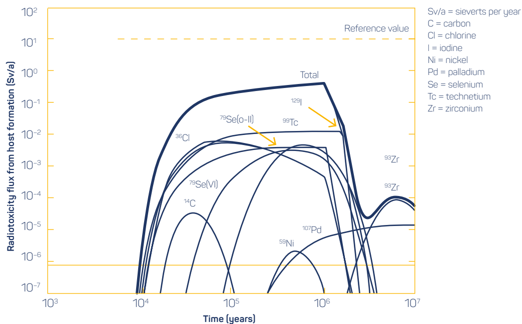
Figure I.38: Comparison of radionuclides released by a geological disposal facility in Boom Clay to those present in agricultural fertilisers, expressed in terms of radiotoxicity
