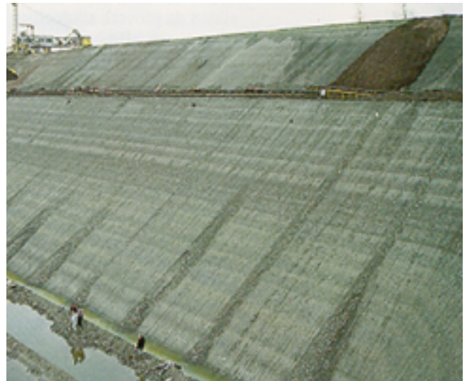
Figure I.35: Uniformity of the Boom Clay formation, as seen where it is exposed at ground level
