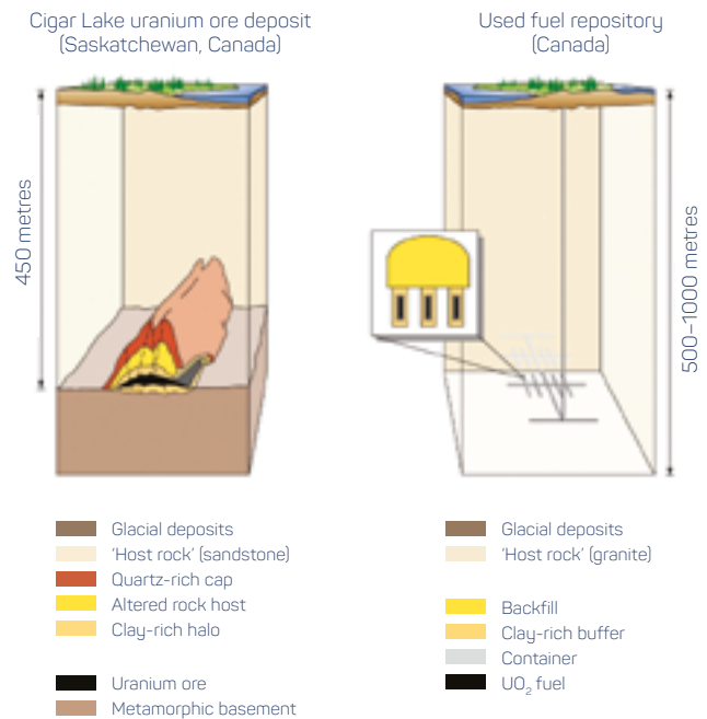
Figure I.8: Cross-section of Cigar Lake uranium ore body, Canada (left), and an early concept for a used fuel GDF (right)
